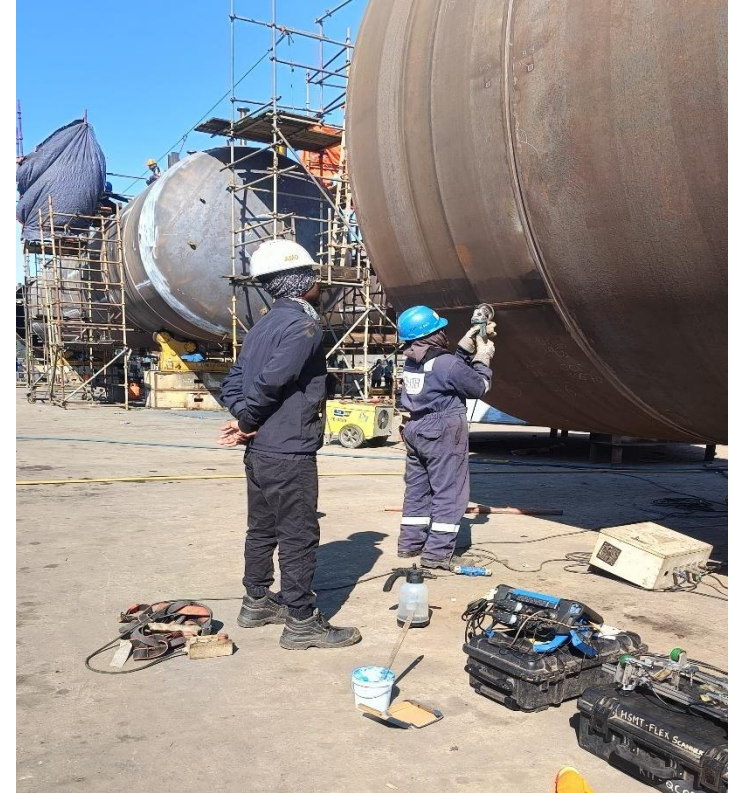
PAUT Inspection of Furnace Pipes and Vessels at Yanbu Aramco Sinopec Refining Company (Yasref) Ltd, Kingdom of Saudi Arabia
